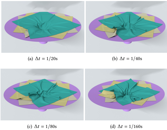
Fig. 14. Funnel. We simulate this example with various time step sizes. While our method reliably handles collisions at a large time step, i.e., \Delta t=1/20s , we recommend using a smaller time step in practice for more accurate results with less numerical damping.
