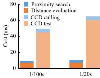
Fig. 10. Comparison with CCD. Overall, the CCD-free stepping schemes for collision handling is five to seven times faster than the CCD-based schemes within a single time step.
