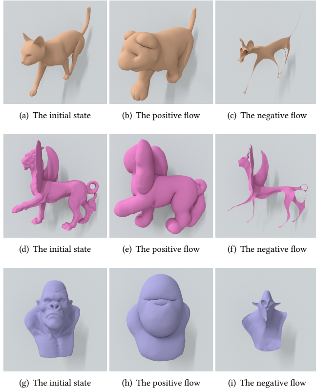
Fig. 16. Globally injective normal flow. Our method can also be applied to enforce global injectivity in both positive and negative normal flows.
