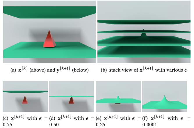
Fig. 9. Termination condition and threshold \epsilon . With the same \mathbf{x}^{[k]} and \mathbf{y}^{[k+1]} , the accumulated moving distance from \mathbf{x}^{[k]} to \mathbf{x}^{[k+1]} is getting close to the distance from \mathbf{x}^{[k]} to \mathbf{y}^{[k+1]} as \epsilon approaching zero, reducing the risk of early termination.
