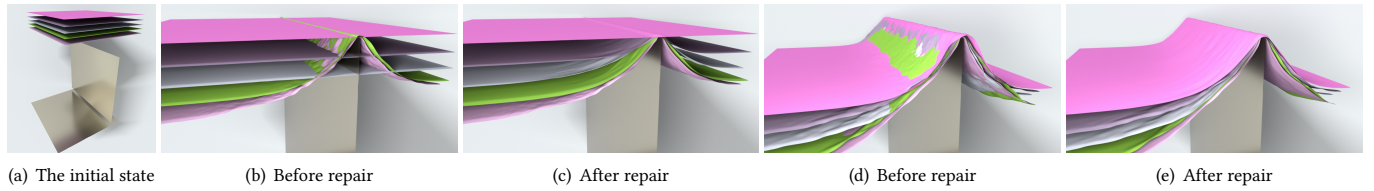
Fig. 15. Cloth and blade colliding. In this example, five square cloth patches are dropped onto a sharp metal blade, and then they drape, slide and stack under gravity. Our method reliably projects severely penetrated frames ((b) and (d)) to intersection-free states ((c) and (e)).
