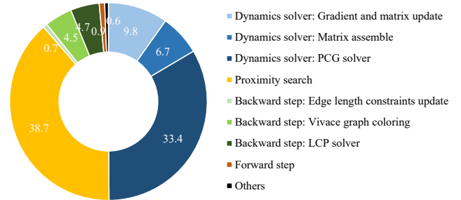
Fig. 13. Breakdown analysis. We visualize a typical breakdown of the cost spent in each stage for the bow knot example. As shown in this figure, the PCG solves and the proximity search are the two most computationally expensive parts in our simulator.
