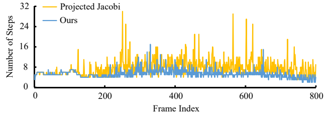
(a) The number of steps fluctuating over frames
