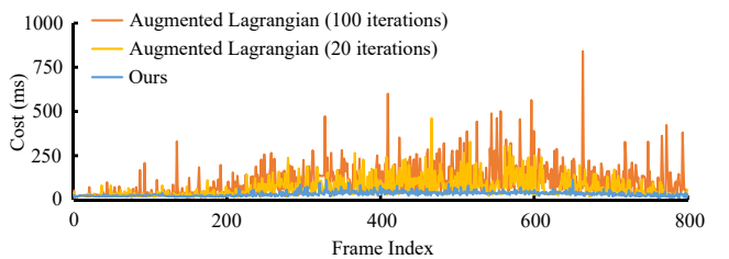
(b) The collision cost fluctuating over frames
