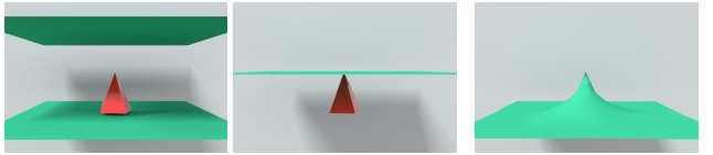
Fig. 3. Linearization choices. The tunneling artifact occurs between two intersection-free states \mathbf{x}^{[k]} and \mathbf{y}^{[k+1]} (Fig. (a)). Projecting \mathbf{y}^{[k+1]} back to \Omega based on the constraints assembled around \mathbf{y}^{(l)} stagnates \mathbf{x}^{[k+1]} (Fig. (b)). Instead, if we assemble and linearize contact constraints around \mathbf{x}^{(l)} , \mathbf{y}^{(l)} manages to cross the boundary of \Omega and stay on the same side as \mathbf{x}^{(l)} , eventually advancing \mathbf{x}^{(l)} to a more reasonable solution (Fig. (c)).
