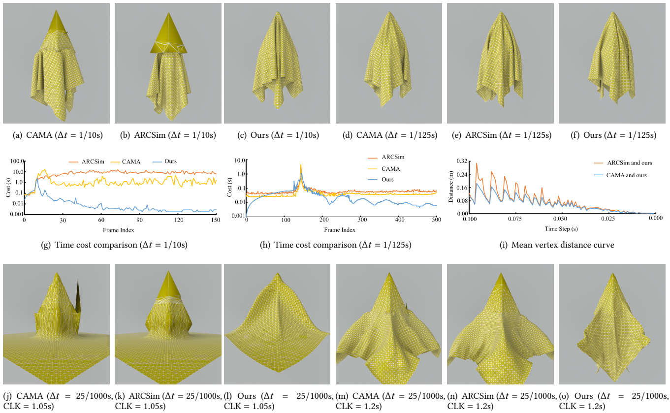
Fig. 19. Robustness to large time steps. A piece of cloth (1m×1m) falling on a sharp cone is simulated with a decreasing time step, from \Delta t=1/10s to \Delta t=1/1000s . Compared to existing impact zone methods such as [Narain et al. 2012; Tang et al. 2016], our method produces nearly artifact-free dynamic simulation even with large time steps, exhibiting superior performance. In contrast, existing methods suffer from visible artifacts until the time step is reduced to a small enough value.
