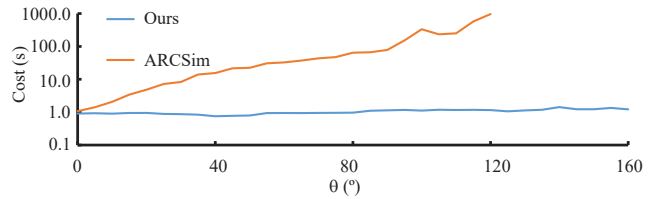
(e) Time cost comparison with ARCSim [Narain et al. 2012]
