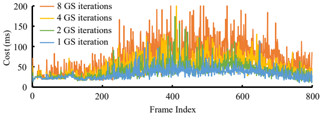
(b) The collision cost fluctuating over frames
