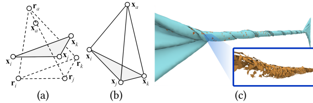
Fig. 4. Vertex-triangle pair. Our constraint enforces the volume of \mathbf{x}_a \mathbf{x}_i \mathbf{x}_j \mathbf{x}_k to be the same as its reference \mathbf{r}_a \mathbf{r}_i \mathbf{r}_j \mathbf{r}_k (Fig. (a)), in which the vertex and the triangle are separated by a threshold distance \delta (Fig. (b)). Tessellated with small tetrahedra in crevices, the simulated cloth robustly prevents self-intersections (Fig. (c)).
