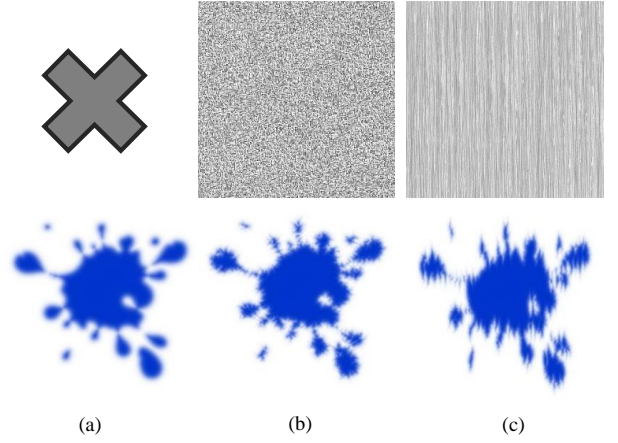
Figure 7: Diffusion Control. Different diffusion effects (bottom) can be created after using different textures (top) to modify the sharpening direction. (a) Isotropic diffusion; (b)(c) Anisotropic diffusion.
