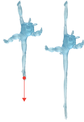
Fig. 3. Comparison with VBD & 2nd SD. The Armadillo model consists of 1M vertices and 3.4M elements. We fix its left hand and drag the right leg downwards to produce a large-scale body deformation. We record the total number of iterations needed for this example using VBD [Chen et al. 2024c], 2nd SD [Lan et al. 2022], and our method under different material stiffness with h = 1/100 . Our method is 15× faster than 2nd SD and 40× faster than VBD. After further increasing the stiffness of the Armadillo by 20 times, our method is 34× faster than 2nd SD, and 137× faster than VBD (VBD switches to a highly conservative time step of h = 1/20000 ).
