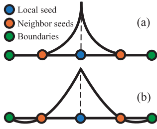
Fig. 6. (a) Anchoring boundary nodes completely results in weight damping. (b) Principal projection yields smoother weight functions.
