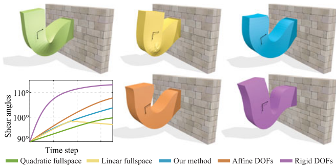
Fig. 3. We apply pure bending moments along the neutral axis of the beam model. The bending quality is measured using the maximum shearing angle along the neutral axis. Our method yields a much smaller shearing locking artifact than other competitors including affine DOFs [10], and rigid DOFs [11]. The ground truth is the result using fullspace quadratic tetrahedral elements. Under such challenging bending test, even fullspace simulation using linear elements will fail.
